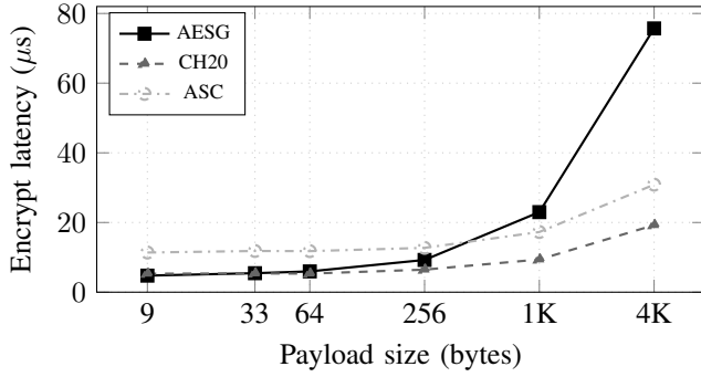
Fig. 1. AEAD encrypt latency versus payload size. CH20 (NEON SIMD) scales at 3.4 \mu\text{s}/\text{KiB} ; AESG at 17.7 \mu\text{s}/\text{KiB} (software table-lookup). Below 64 B, setup cost dominates and ciphers converge.
